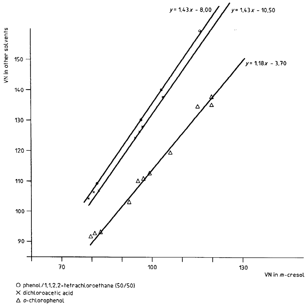
Figure A.2 — Viscosity number of PBT in m -cresol relative to that in other solvents
