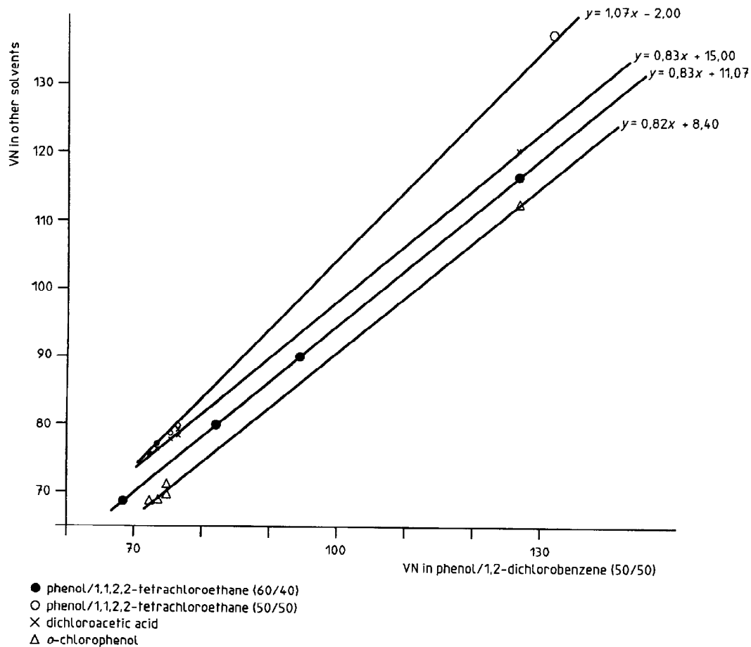
Figure A.1 — Viscosity number of PET in phenol/1,2-dichlorobenzene (50/50) relative to that in other solvents
